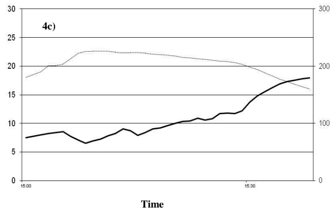
Fig.4– Evolution of combustion process in April 3. Figs.4a), 4b) and 4c), concern to time periods 9h54m-10h40m, 10h40m-15h and 15h-15h38m, respectively.
