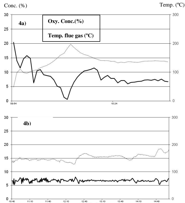
Fig. 3 - Evolution of straw combustion in 3 April trial concerning to the time variation of 3 variables.
